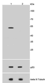
Fig. 1. Western blot analysis of Acetyl-p53 (Lys370) on HepG2 cell lysates using anti-Acetyl-p53 (Lys370) antibody at 1/1,000 dilution. Positive control: Lane 1: HepG2 treated with Etoposide 20uM and Trichostatin A 500 nM for 6 hours whole cell lysates; Lane 2: HepG2 untreated whole cell lysates
